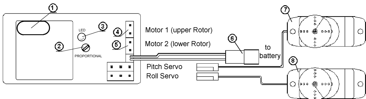
Fig. (3): Connection of the "4 in 1" control box
